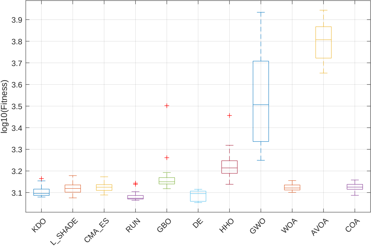
CEC2017 F11 (Numerical) - Boxplot
